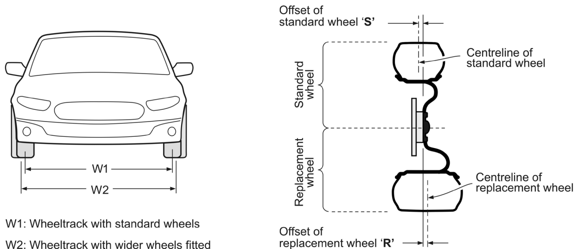
FIGURE 1: WHEELTRACK AND WHEEL OFFSET
